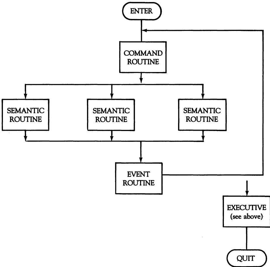
Figure 17.2 General flow diagram of adventure game
